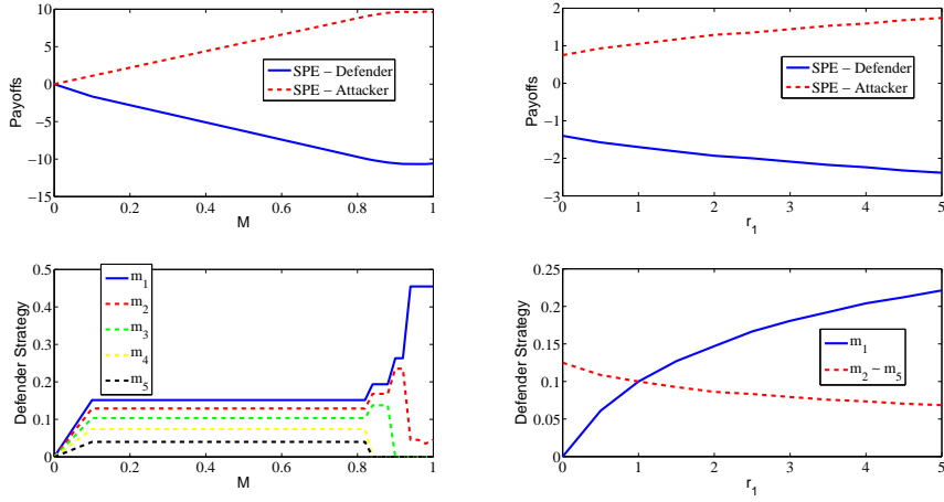
Fig. 3: The effects of varying resource constraints and r_1 , where w = [2 \ 2 \ 2 \ 2 \ 2] , C^D = C^A = [1 \ 1 \ 1 \ 1 \ 1] , B = 0.5 , r = [5 \ 4 \ 3 \ 2 \ 1] in (a), r = [r_1 \ 1 \ 1 \ 1 \ 1] and M = 0.3 in (b).
